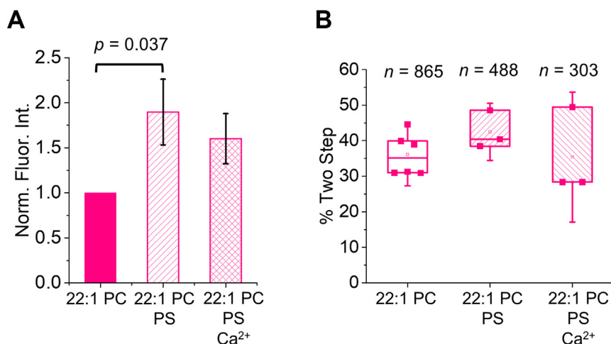
Figure 5. PS interactions with TMJM in thick bilayers. A, normalized fluorescence intensities from emission spectra of TMJM in 22:1 PC liposomes with 10% POPS and 5 mM Ca 2+ . Bars are means \pm SD, n = 3 . p -value was determined by Mann-Whitney U test. B, percentages of dimeric TMJM from SM-phobleaching experiments in 22:1 PC examining effects of 10% POPS and 1 mM Ca 2+ . Data are from three to six independent experiments. n is number traces counted for each. No statistically significant differences were found.
